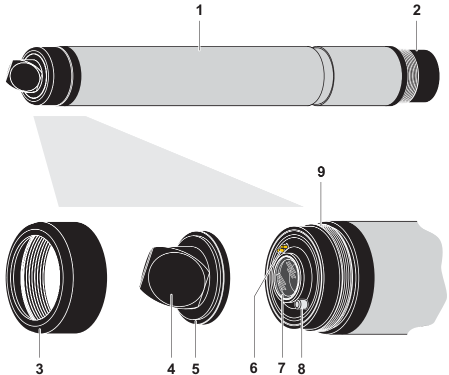
Fig. 1-2 Structure of the D. O. sensor
